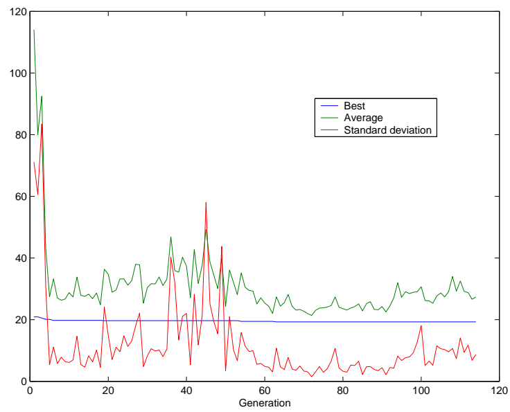
Figure 9: Evolution of pricing error.
