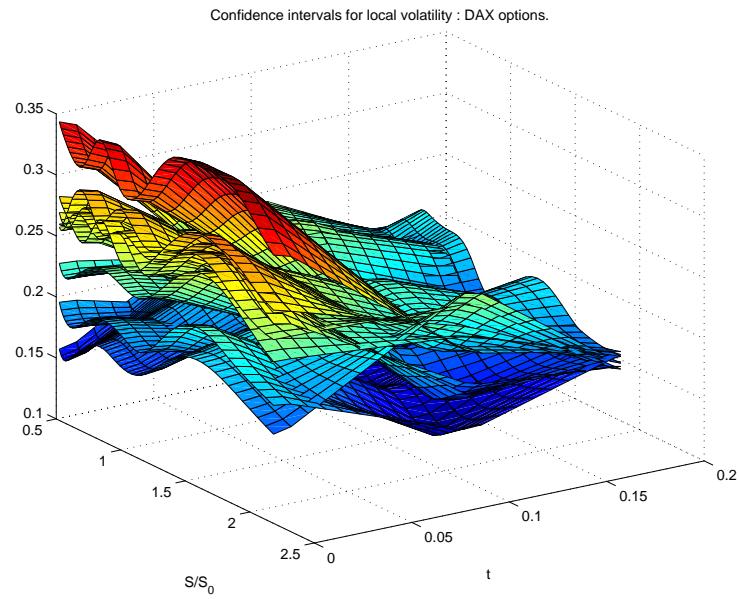
Figure 13: Uncertainty on local volatility surfaces: DAX options.
