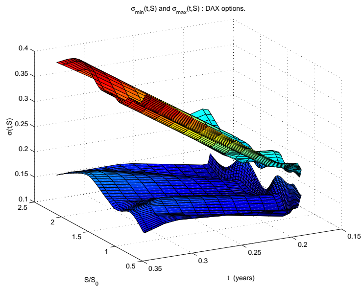
Figure 14: Pointwise lower and upper bounds for the local volatility \sigma_{\min}(t, S) and \sigma_{\max}(t, S) computed from 10 best solutions, DAX options.
