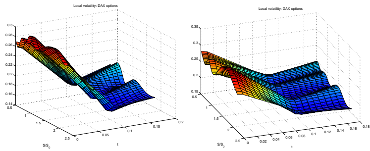
Figure 10: Local volatility surfaces: DAX options.
