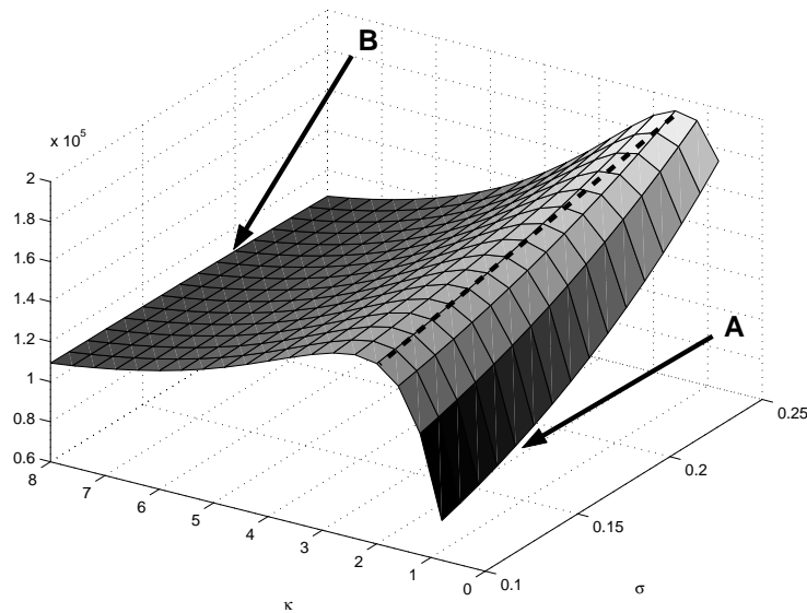
Figure 3: Error surface for Variance Gamma (pure jump) model, DAX options.
