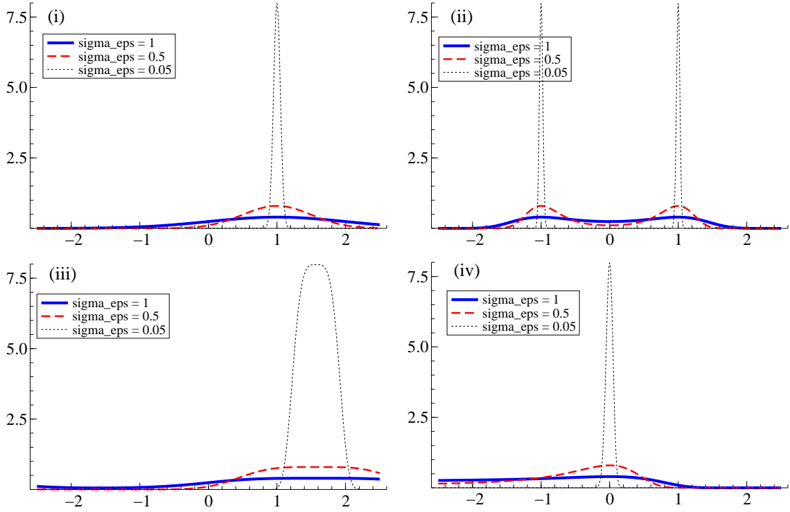
Figure 3: Incremental weight functions \tilde{w}_n for three different levels of measurement error. \sigma_\varepsilon = 1, \sigma_\varepsilon = 0.5, \sigma_\varepsilon = 0.05 . We observe \mathbf{y}_n = 1 . Each panel plots a different functional form: (i) h(\mathbf{x}_n) = \mathbf{x}_n ; (ii) h(\mathbf{x}_n) = \mathbf{x}_n^2 ; (iii) h(\mathbf{x}_n) = \sin(\mathbf{x}_n) ; and (iv) h(\mathbf{x}_n) = \exp(\mathbf{x}_n) .
