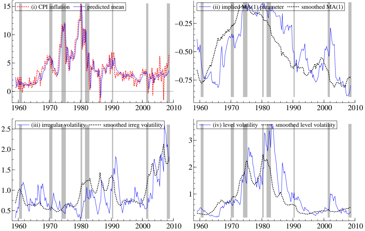
Figure 4: Estimates from the time-varying local level model applied to quarterly U.S. inflation Q1:1959-Q3:2008: (i) inflation and its one-step ahead forecast; (ii) filtered and smoothed estimates of the implied MA(1) parameter; (iii) filtered and smoothed estimates of the irregular volatility \exp(\mathbf{x}_{2,n}/2) ; (iv) filtered and smoothed estimates of the state volatility \exp(\mathbf{x}_{3,n}/2) . NBER recession dates are indicated by the vertical bars.
