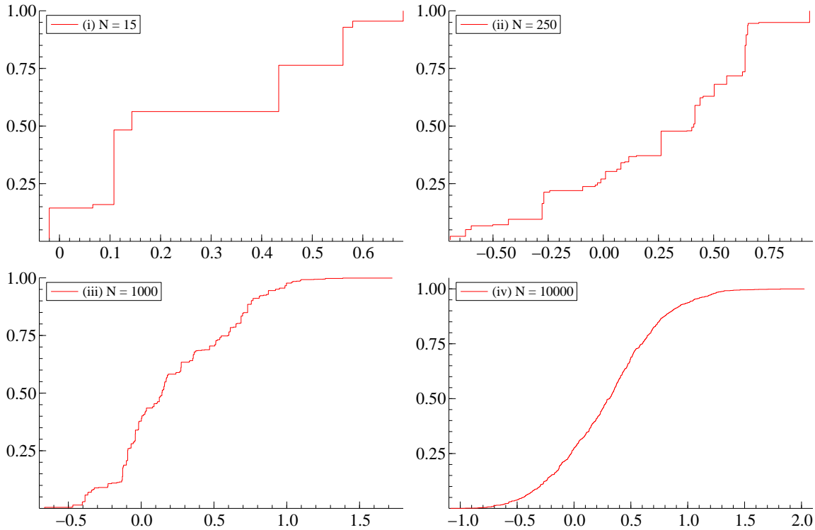
Figure 2: Empirical distribution functions created using the particles to approximate the marginal filtering distribution p(\mathbf{x}_{50}|\mathbf{y}_{1:50};\theta) for the stochastic volatility model. (i) N = 15 particles; (ii) N = 250 particles; (iii) N = 1000 particles; and (iv) N = 10000 particles.
