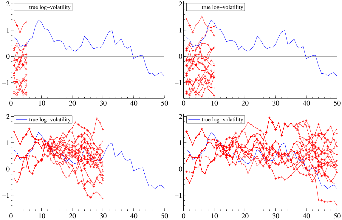
Figure 1: 50 iterations of a discrete-time log-normal stochastic volatility model. Pictured is the true log-volatility (solid line) and a particle system with N=15 particles after: (i) 5 time-steps; (ii) n = 10 time-periods; (iii) n = 30 time-periods; and (iv) n = 50 time-periods.
