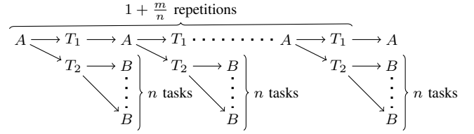
Fig. 4: A task graph for which HeteroPrioDep does not achieve a constant approximation ratio.
