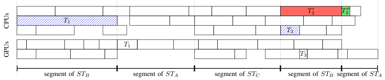
Fig. 3: Different segments of a modified HeteroPrioDep schedule. Aborted tasks are depicted in pattern boxes. GPU is the favorable resource for tasks T_1 , T_2 and T_3 . T_2 completes on its unfavorable resource in the original HeteroPrioDep schedule, hence it is replaced with T_2' and T_2'' in the modified schedule.
