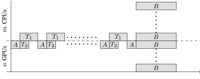
Fig. 6: A better schedule for the task graph of Fig 4.
