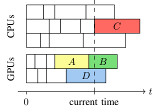
(b) HeteroPrioDep schedule when task C is first scheduled.
