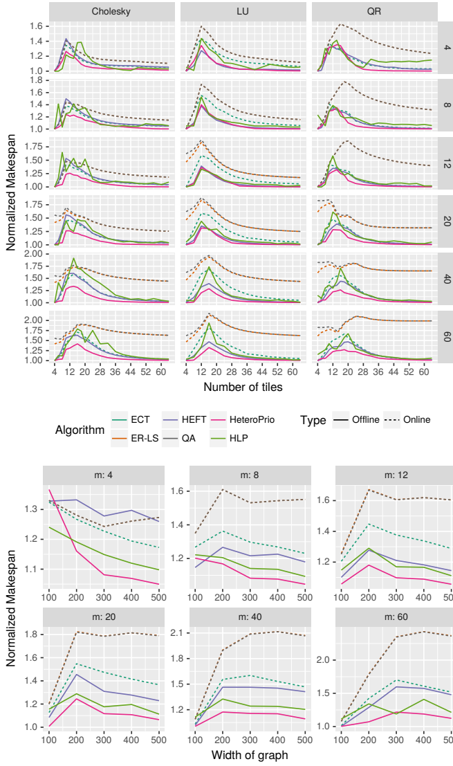
Fig. 8: Comparison of HeteroPrioDep with offline and online algorithms from the literature. Top: Chameleon instances, bottom: fork-join task graphs.
